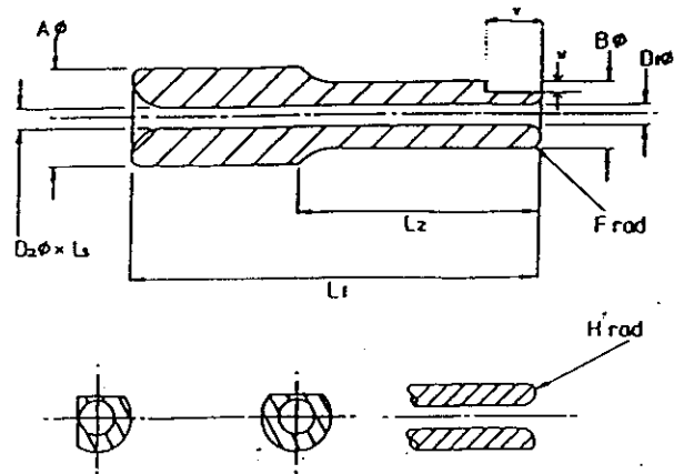
Nozzle Tube "Type Cutter 1" Flat grinded to max. 4 side cutter
