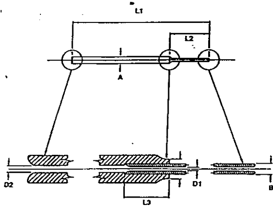
Two Part Tube "Type S2" minimum bore on max. outer diameters.
