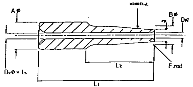
Nozzle Tube "Type S-Angle" Grinded to extreme rejuvenate diam on max. material strength.
