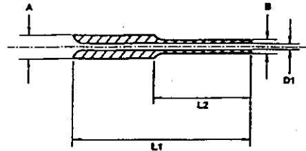
Nozzle Tube "Type S"
